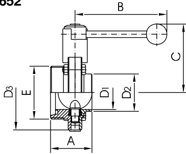
Scheibenventil DIN-GS butterfly valve-DIN-male/welding end
